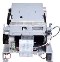
Metallic Printer Enclosure
